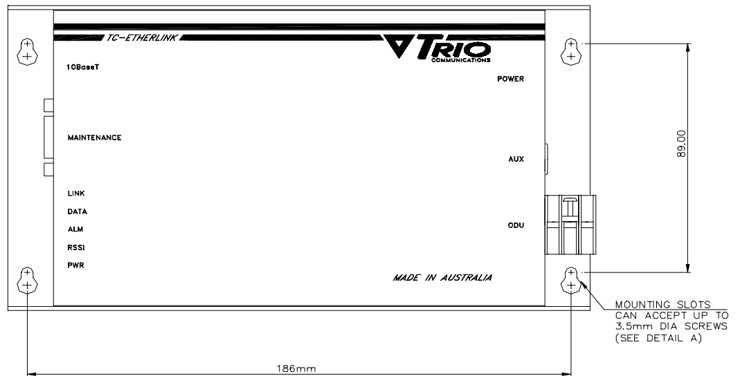
Figure 9 – ITU mounting plate dimensions (not to scale)
