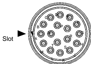
Figure 3 – 17 pin connector
