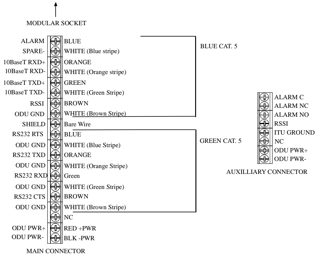
Figure 8 – Terminal Blocks (viewed from top)
