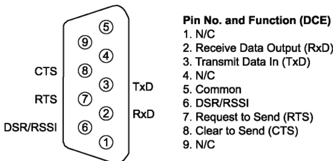
Figure 6 – RS232 Maintenance Port
