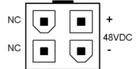
Figure 4 - Power Connector (as viewed from front of socket)
